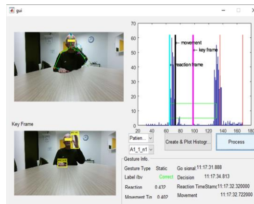
Figure 1. The user interface of our framework
